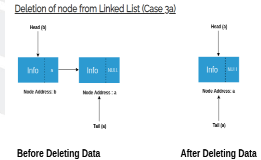
Snapshot 2 : To Deleting a Node
